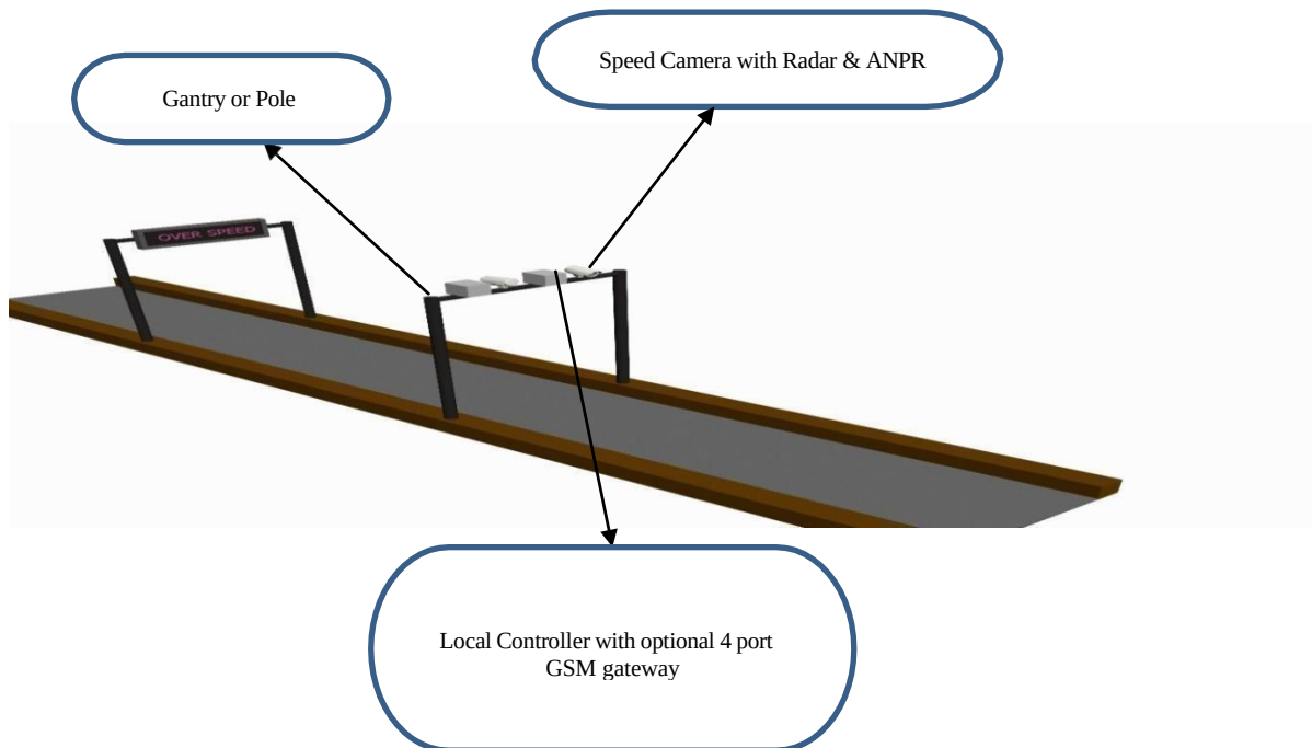
Figure 42. Equipment for ASES
