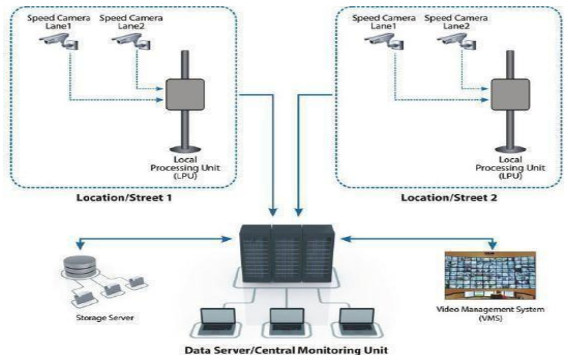
Figure 41. System Architecture
